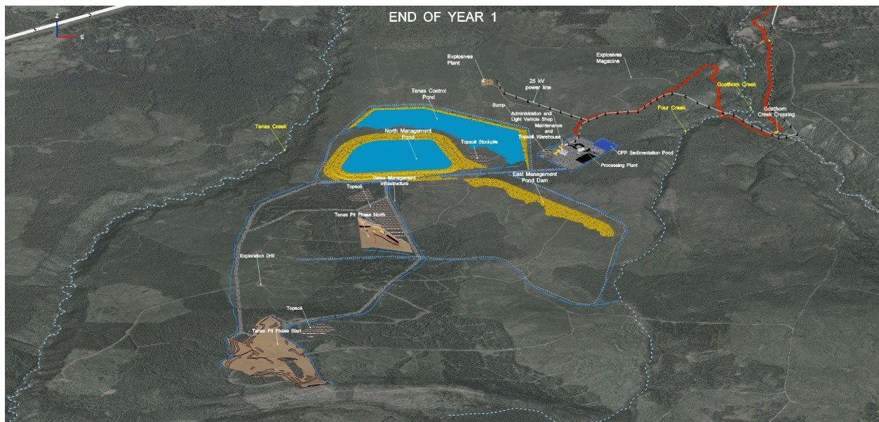
Figure 3: Road plan at the end of Year 1
