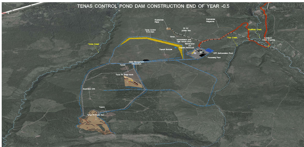
Figure 1: Road Plan at the end of Year -0.5
