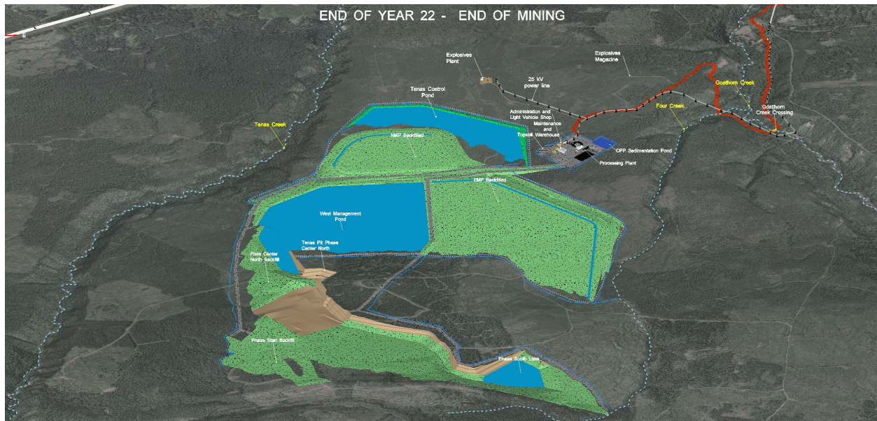
Figure 10: Road plan at the end of active mining
