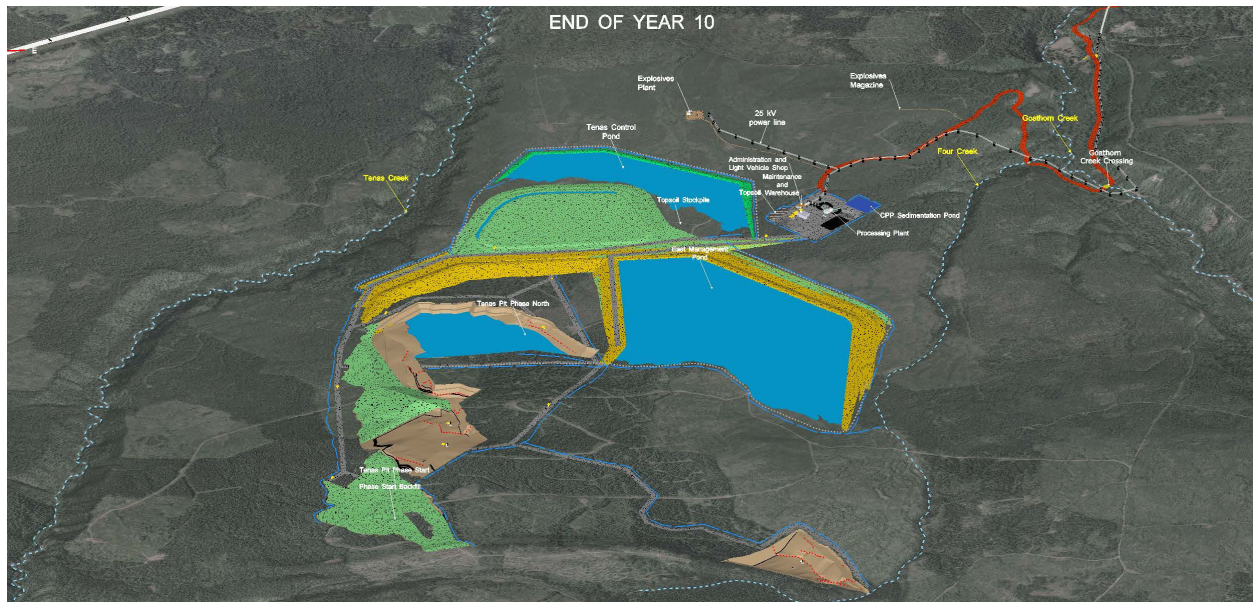
Figure 8: Road plan at the end of Year 10
