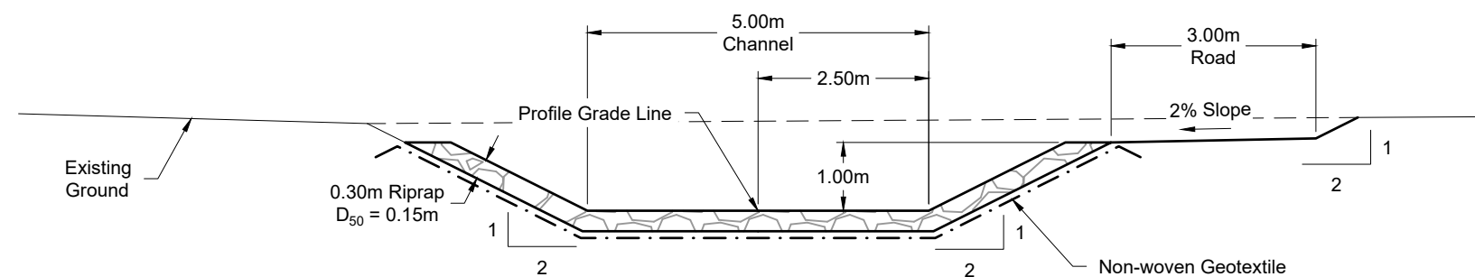
Channel and Road in Cut
