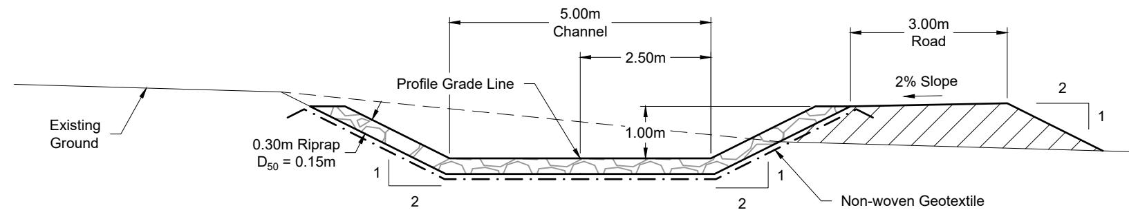
Channel in Cut and Road in Fill
