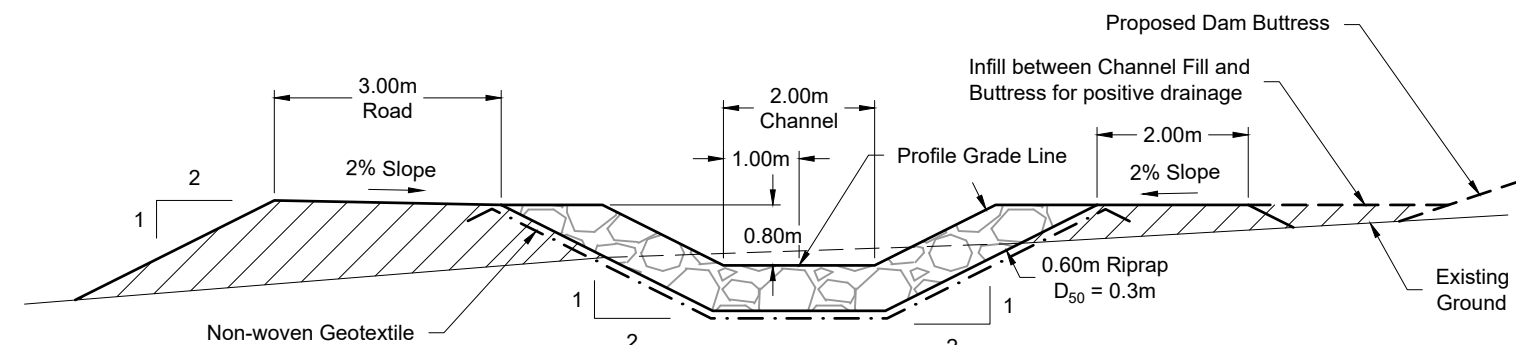
Channel in Cut and Road in Fill
