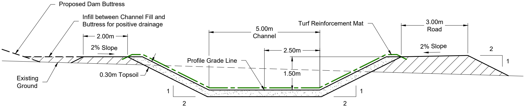
Channel and Road in Fill
