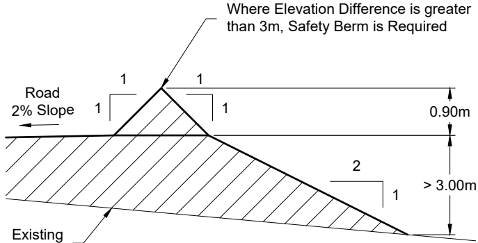
Safety Berm Detail Not To Scale
