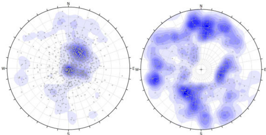
Figure 7-12: Stereographic Projection of ATV data of T18-07D. (Left: All Data; Right: Bedding Poles Removed to show any other joint concentrations)
