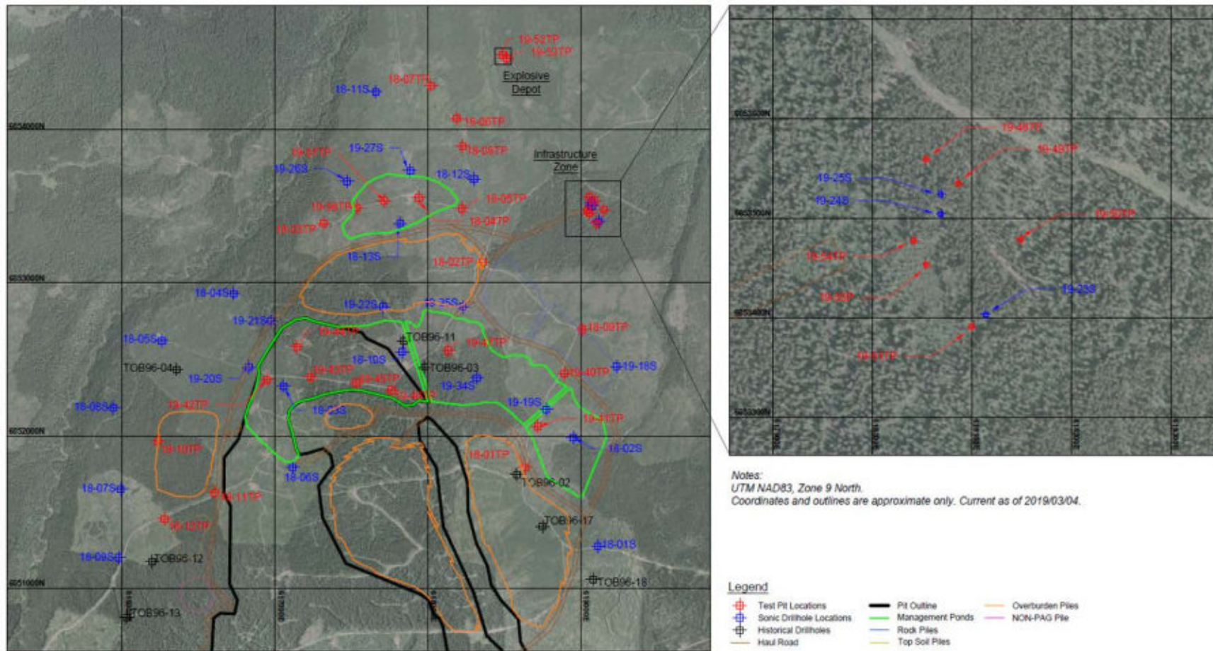
Figure 5-1: Location plan showing 2018, 2019 and historic sonic drillholes and test pit investigations
