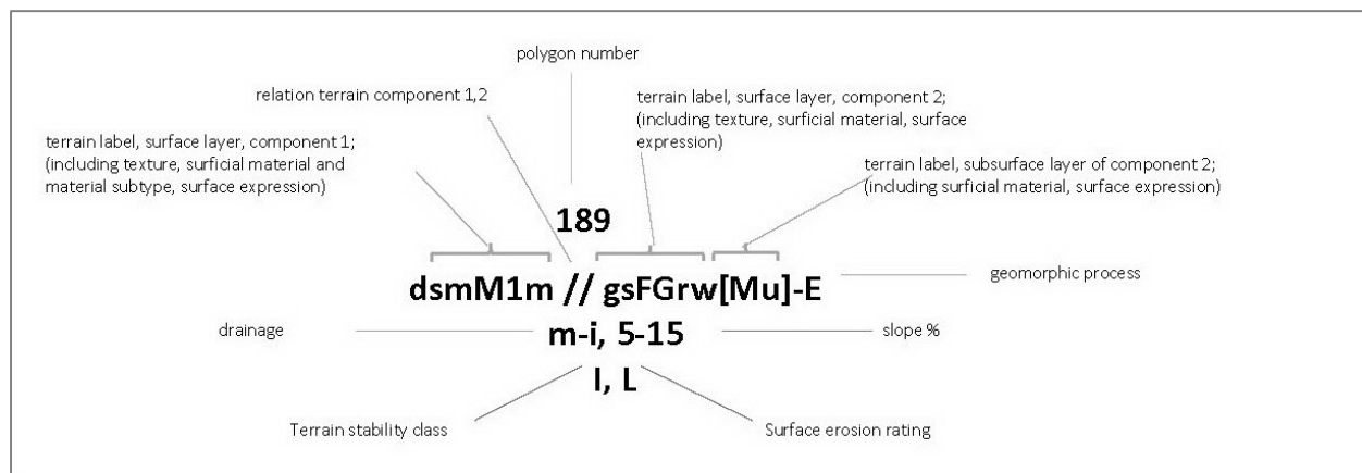
Figure 2-3: Example terrain stability polygon label.
