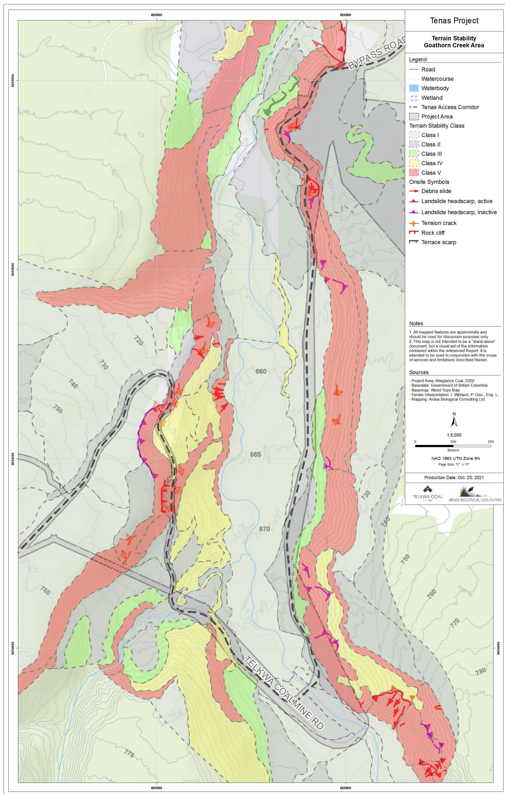
Figure 2-7: TSC IV and V and landslide sites in the Goathorn Creek valley along the Coalmine Road and Caribou FSR.
