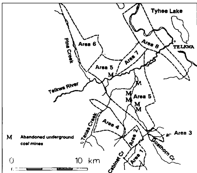
Figure 2 B. Ryan 1993, Showing 8 of 10 areas of Telkwa Coal
